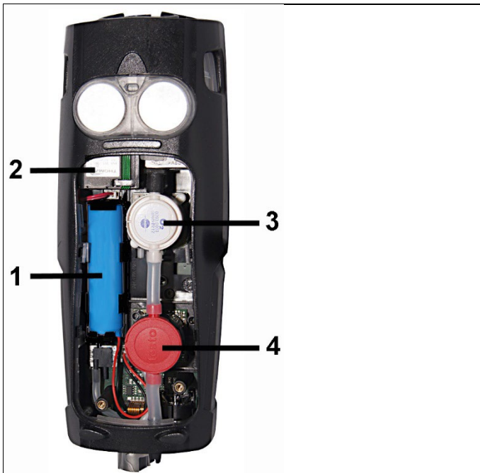
1 Rechargeable battery
